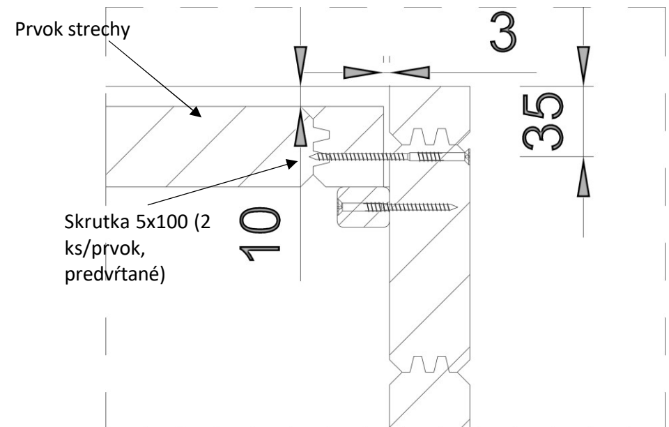
CUT A-A-DETAIL
