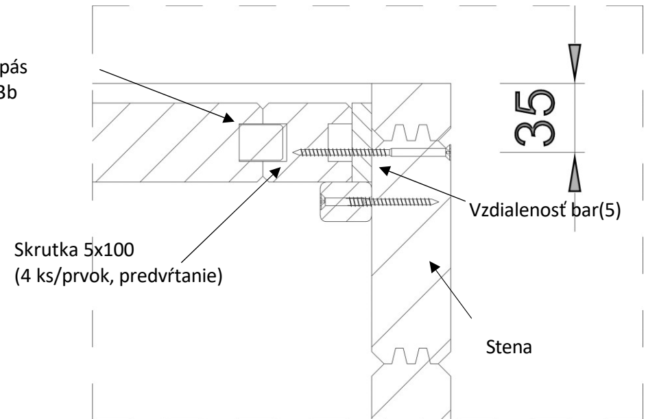
ODDIEL B-B-DETAIL
