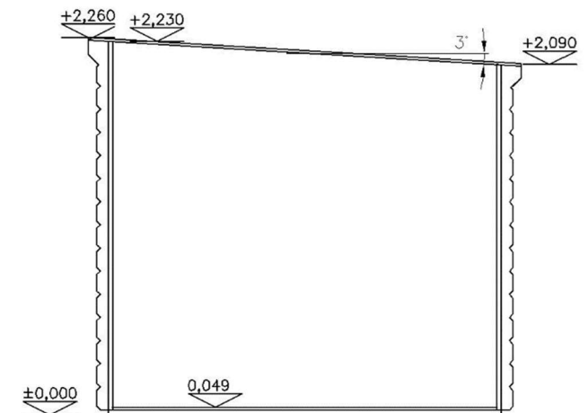
REZ
